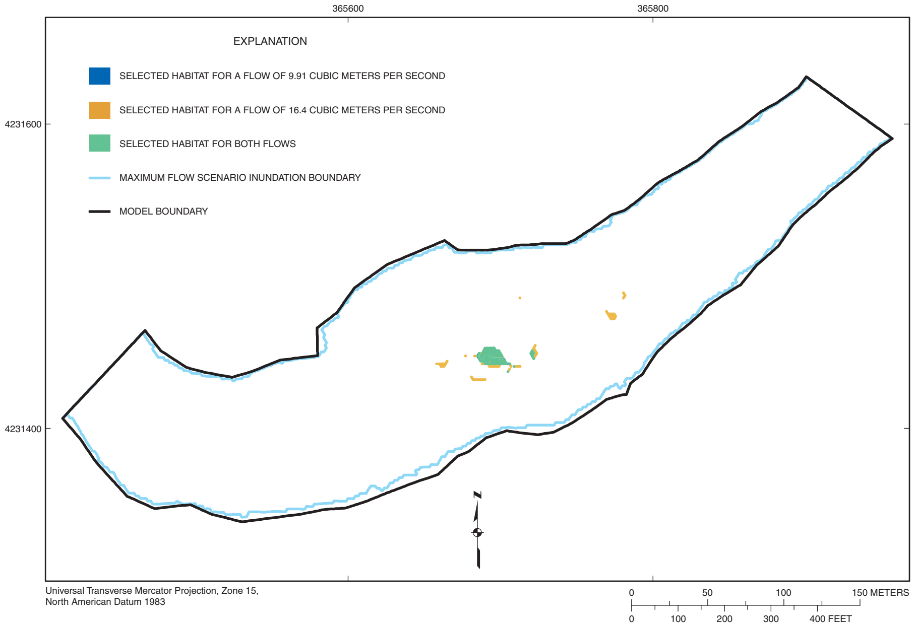
Figure 4-15. Selected habitat area distribution for habitat categories 4, 5 combined (slenderhead darter) at flows of 9.91 and 16.4 cubic meters per second at Marais des Cygnes River site MDC2.
